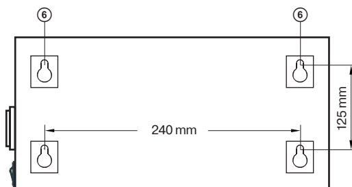
Fig. 2. Rear panel
