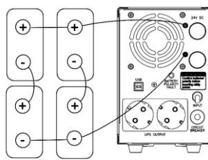
Fig.4 24VDC
