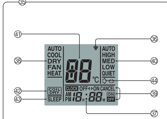
Fig. 7 To facilitate explanation, the accompanying illustration has been drawn to show all possible indicators; in actual operation, however, the display will only show those indicators appropriate to the current operation.
