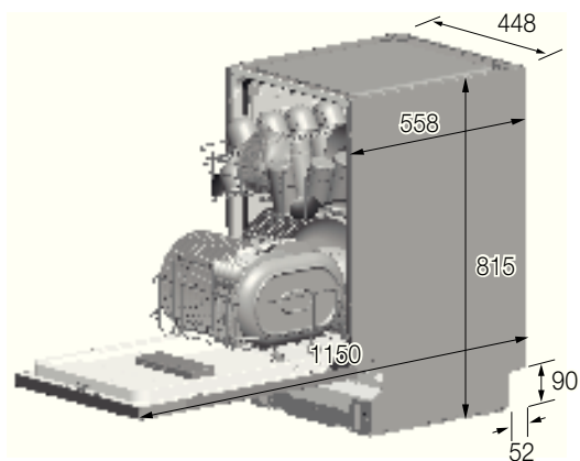
DW50K4050BB / DW50K4030BB
