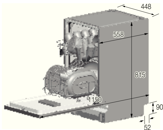
DW50K4050BB / DW50K4030BB
