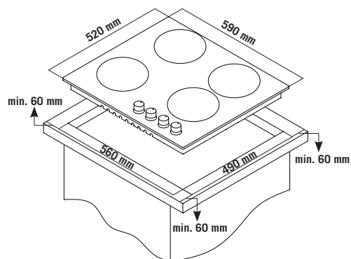
Cooktop Of 60cm
