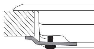
Hooking position for top H=30mm
