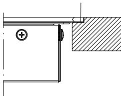
POSITION OF SEALANT IN THE FLUSH WITH TOP VERSION
