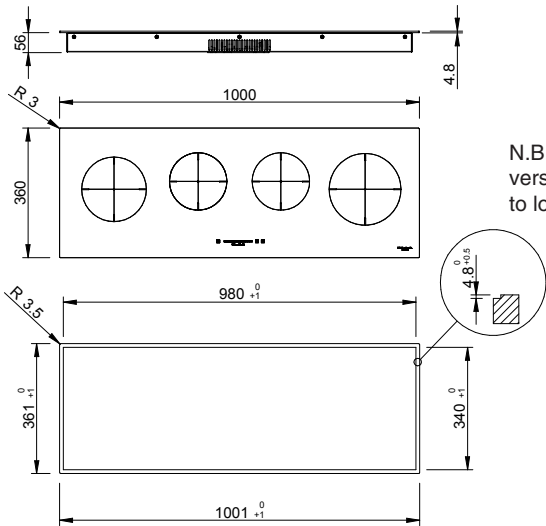
POSITION OF SEALANT IN THE FLUSH WITH TOP VERSION
