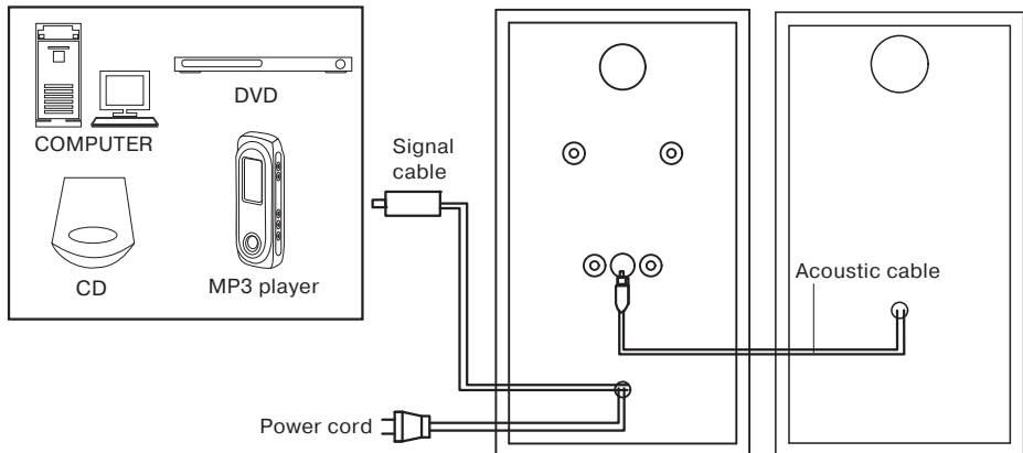
Fig. 2. Connection diagram
