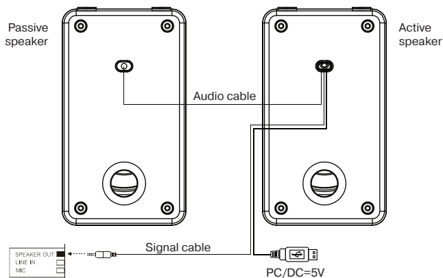
Fig. 2. Connection diagram
