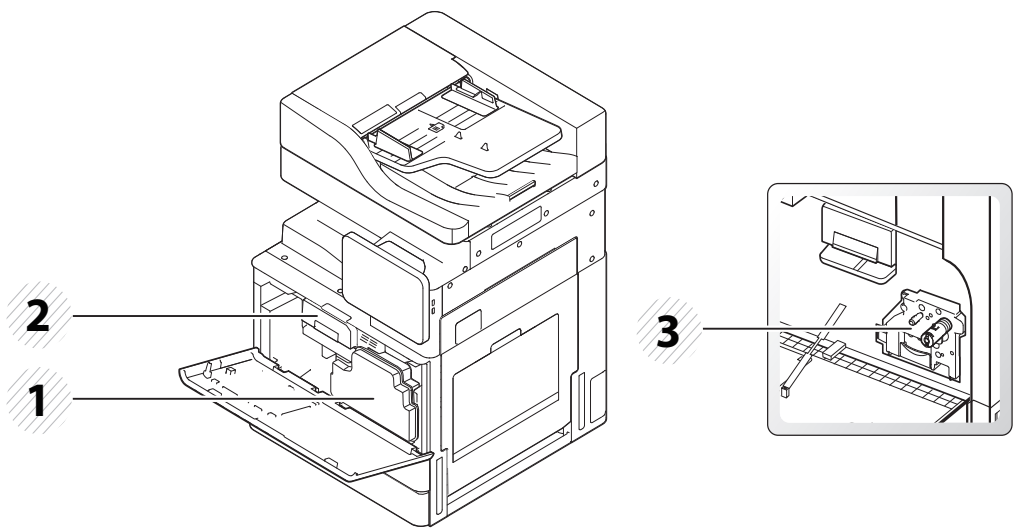
Вид изнутри (K425x series/K430x series/K435x series)
