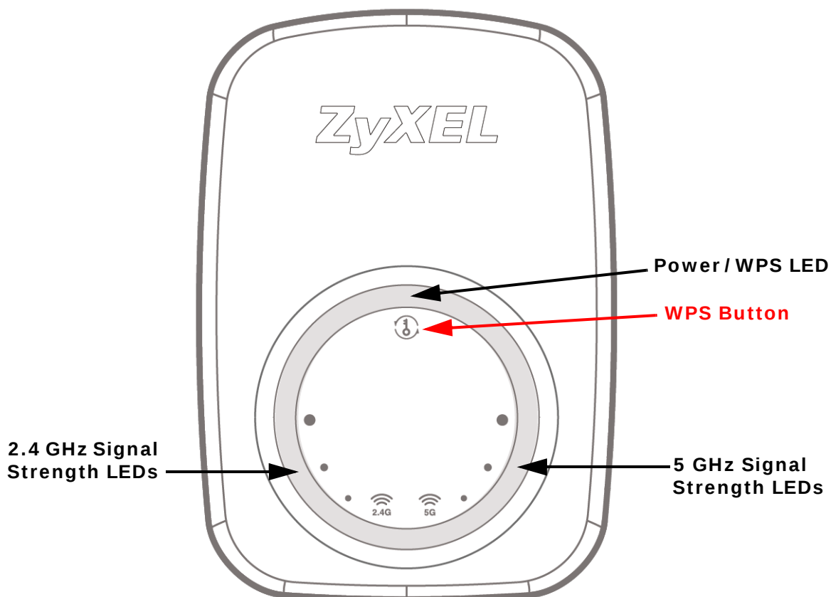
Figure 2 Front Panel
