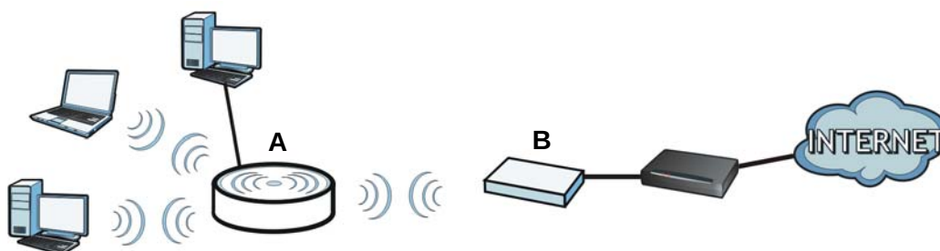
Figure 10 Repeater Mode
