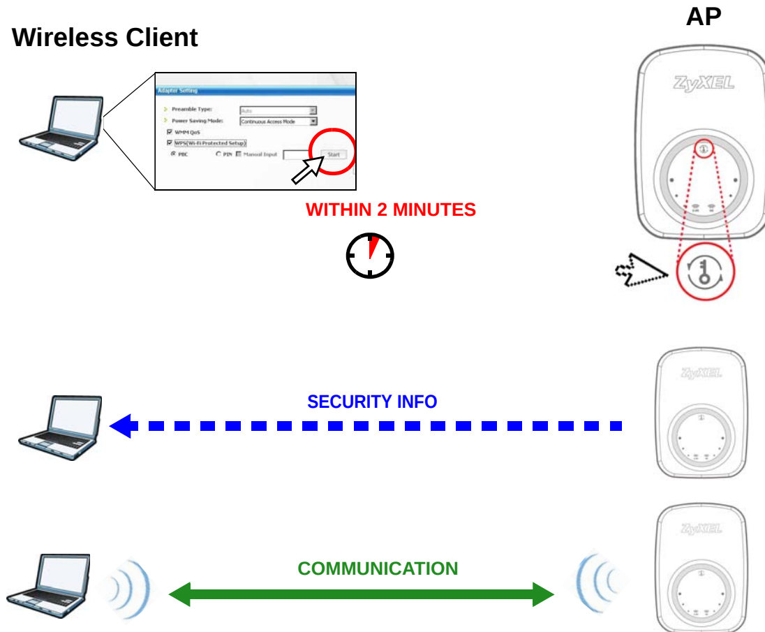
Figure 18 Example WPS Process: PBC Method
