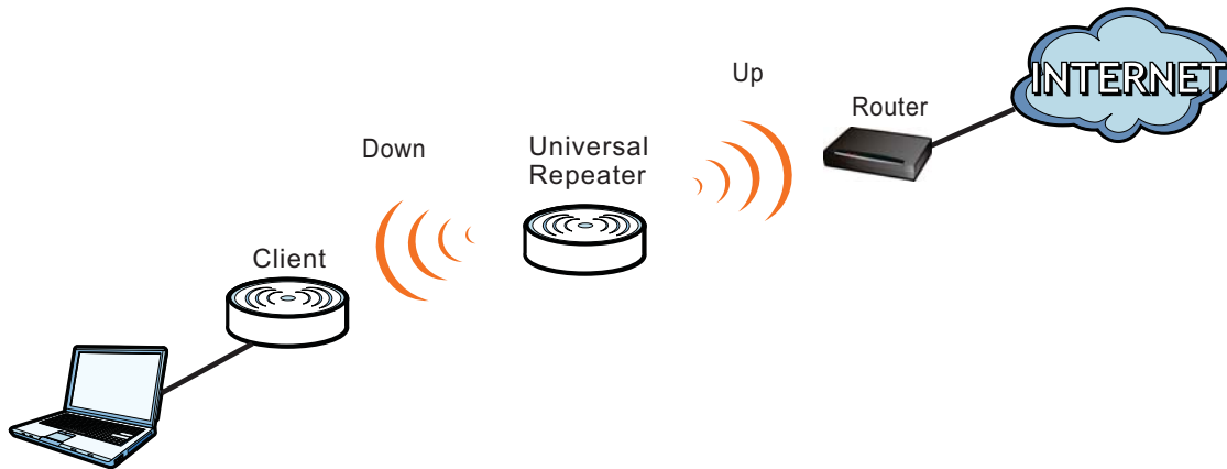
Figure 57 Normal Mode with Up and Down Broadcasting
