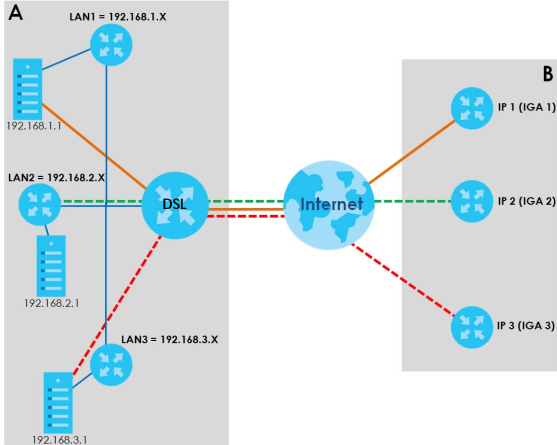
Figure 113 NAT Application With IP Alias
