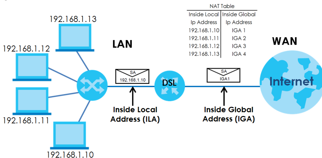
Figure 112 How NAT Works
