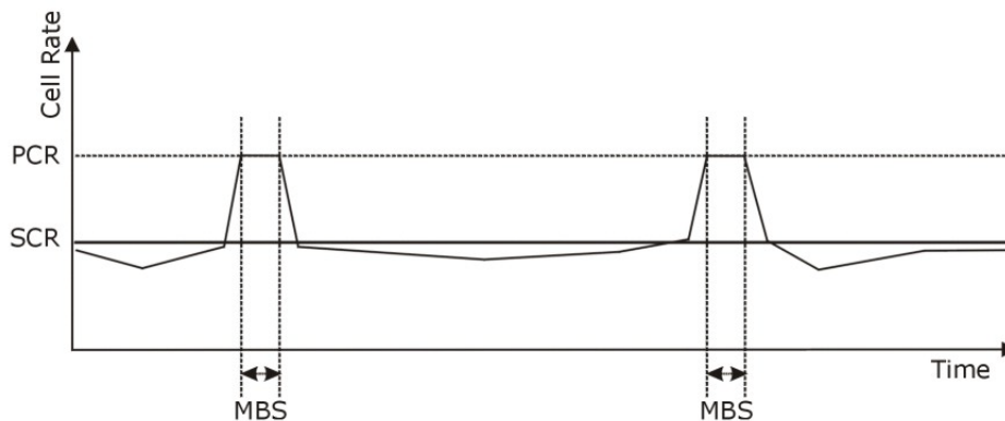
Figure 55 Example of Traffic Shaping
