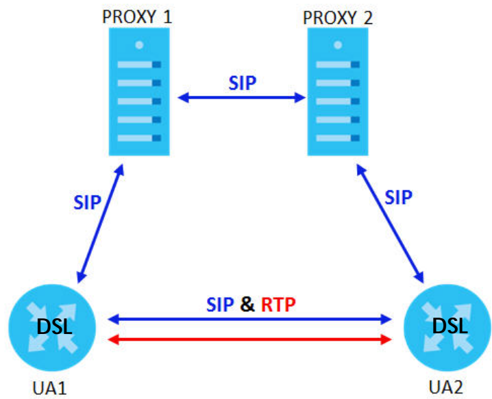
Figure 169 SIP Call Through Proxy Servers
