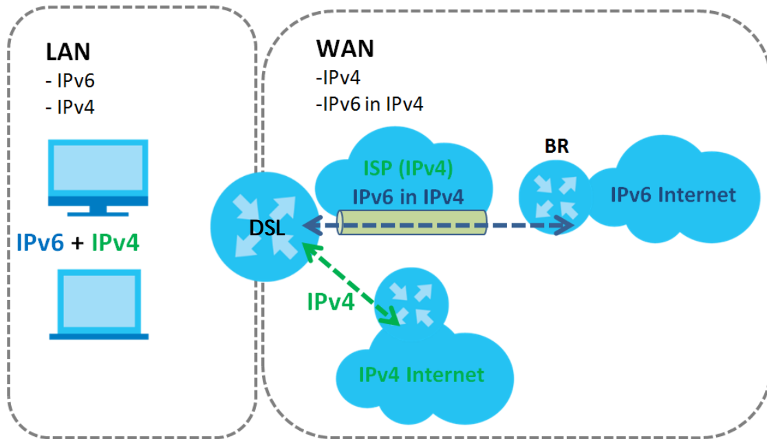
Figure 45 IPv6 Rapid Deployment
