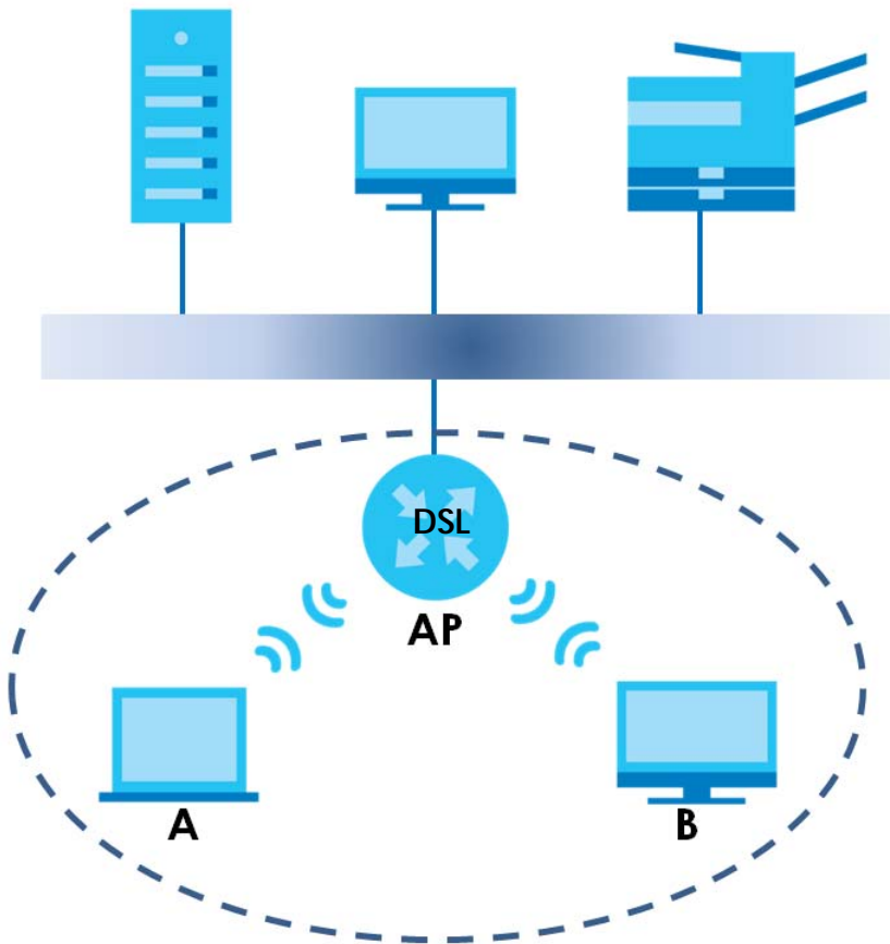
Figure 212 Basic Service Set
