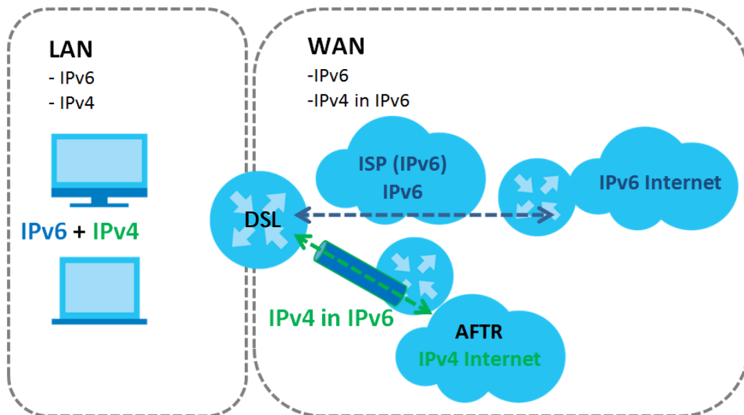
Figure 46 Dual Stack Lite
