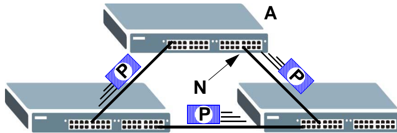
Figure 65 Loop Guard - Network Loop
