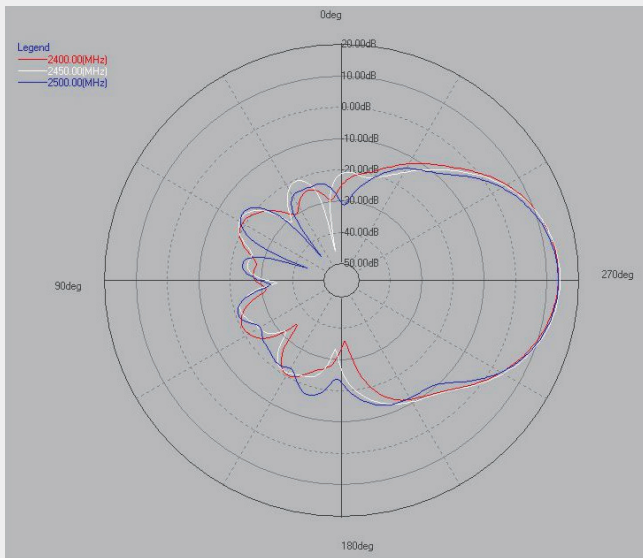
2.4G (PHI=0)
