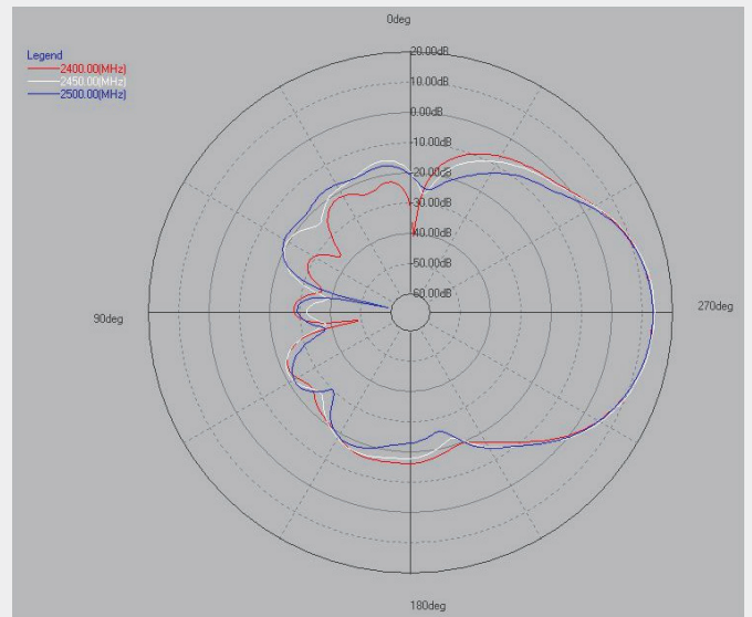
2.4G (PHI=90)
