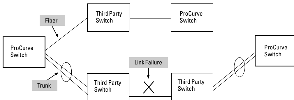
Figure 10-20. UDLD Example
