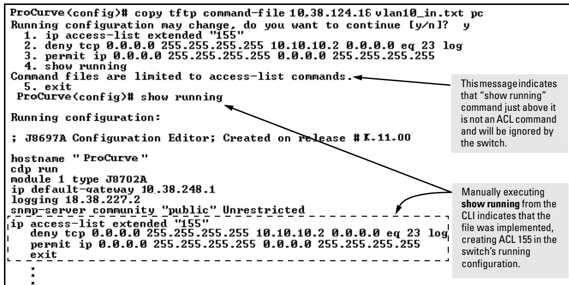
Figure A-11. Example of Using the Copy Command to Download and Configure an ACL
