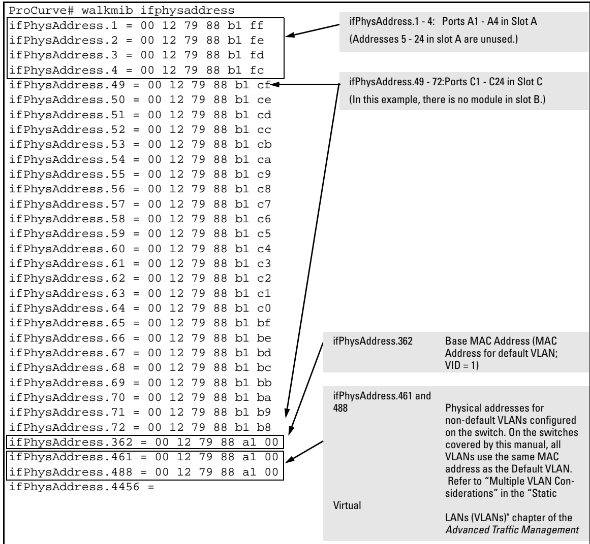
Figure D-2. Example of Port MAC Address Assignments on a Switch
