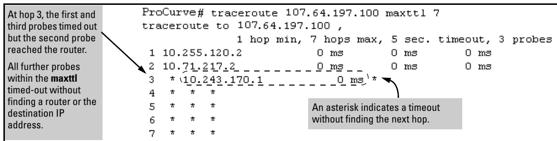
Figure C-25. Example of Traceroute Failing to Reach the Destination Address
