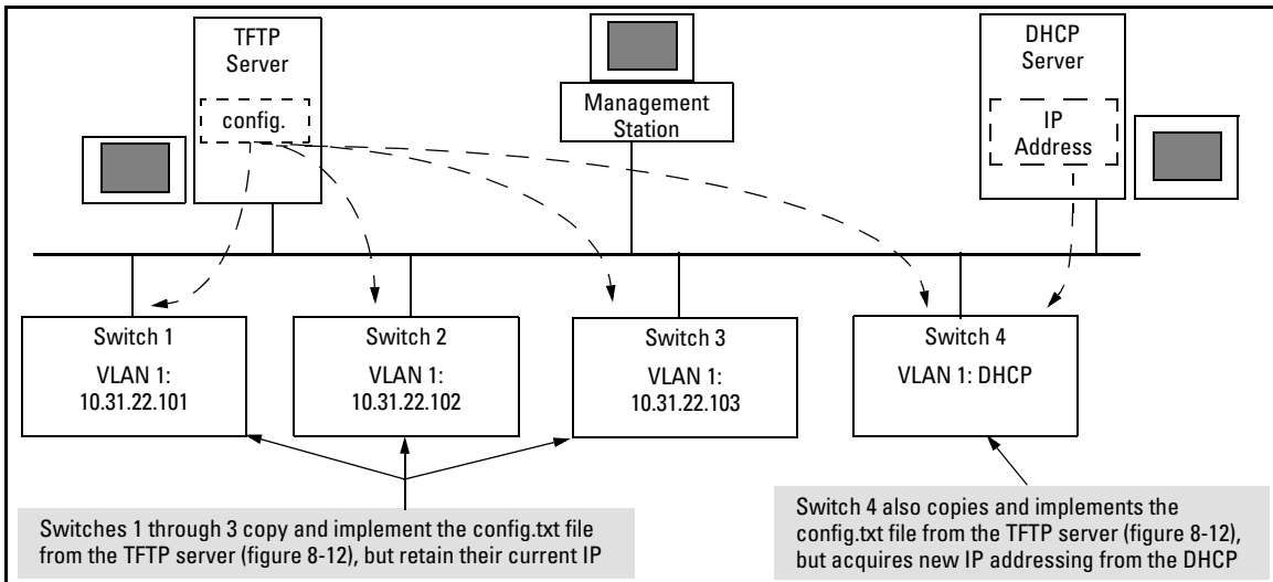
Figure 8-11. Example of IP Preserve Operation with Multiple Series Switches
