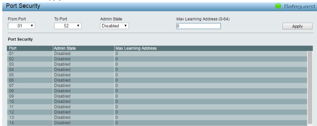
Figure 4.100 – Security > Port Security
