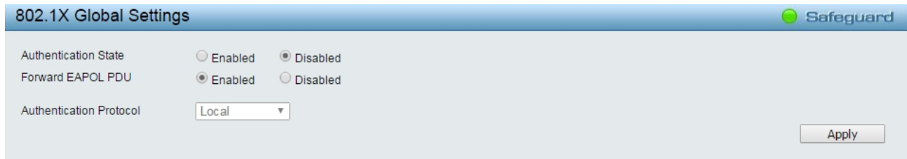
Figure 4.118 – AAA > 802.1x Global Settings
