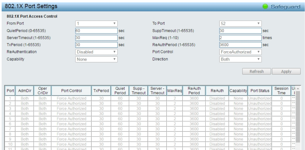
Figure 4.119 – AAA > 802.1X > 802.1X Port Settings
