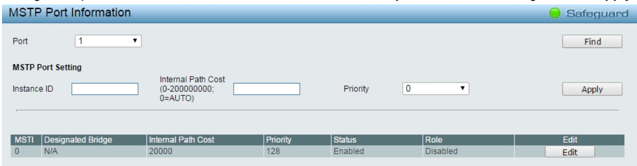
Figure 4.60 – L2 Functions > Spanning Tree > MST Port Information
