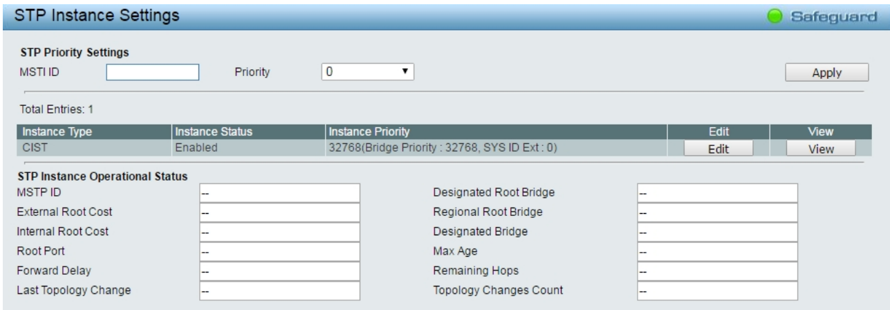
Figure 4.59 – L2 Functions > Spanning Tree > STP Instance Settings
