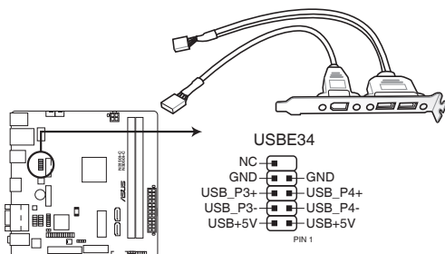
N3150I-C / N3050I-C USB2.0 connector
