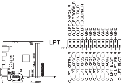
N3150I-C / N3050I-C Parallel port connector
