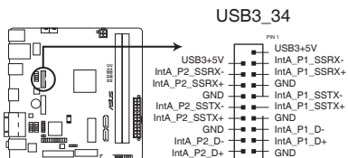
N3150I-C / N3050I-C USB3.0 connector
