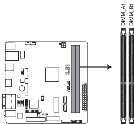
N3150I-C / N3050I-C 240-pin DDR3 DIMM sockets
