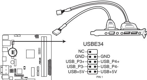
N3150I-C / N3050I-C USB2.0 connector
