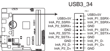
N3150I-C / N3050I-C USB3.0 connector
