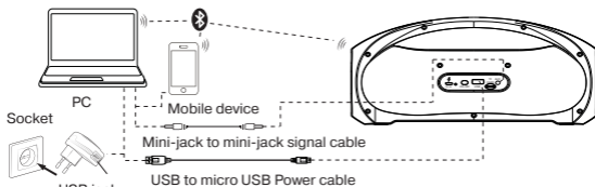
Fig. 4. Connection diagram
