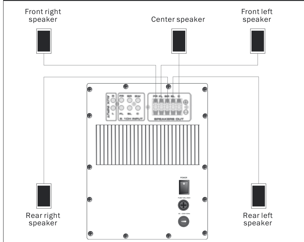
Connection of subwoofer to the satellite speakers and the center speaker
