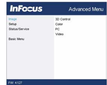
Advanced Menu
